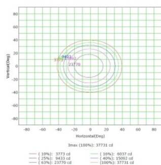
Isocandela (rectangle)
